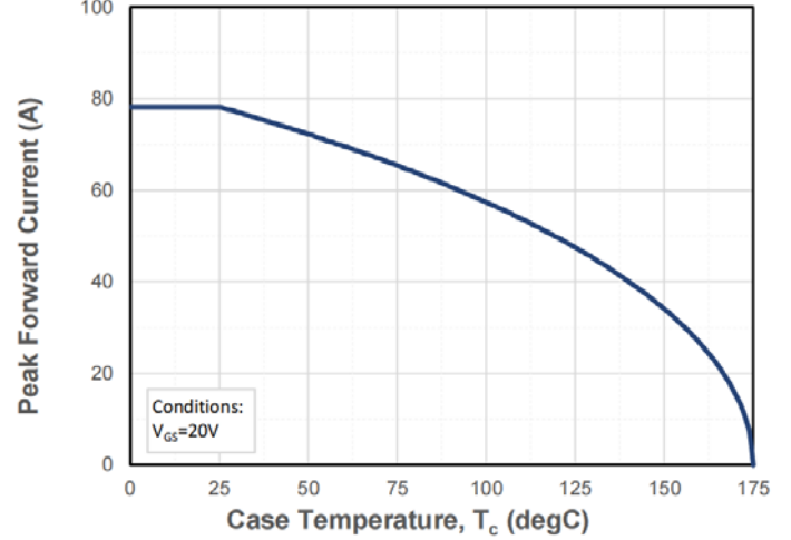
Figure 14. Drain Current Derating vs. Case Temperature
